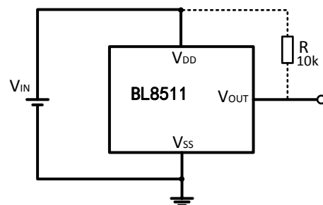
(2) Detector threshold test circuit
